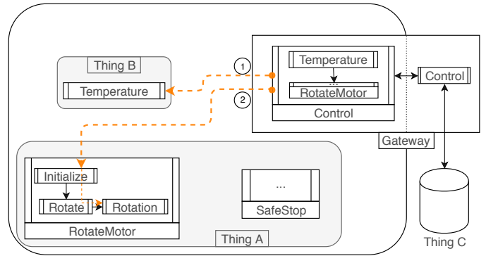
Figure 6: A gateway can compose a system through the use of the path vocabulary. Here, the system is a temperature control system with a temperature sensor and an industrial ventilator. Things, such as Thing C, that do not have physical access to the system components can execute simple Thing Description interactions to interact with the system through the gateway.
